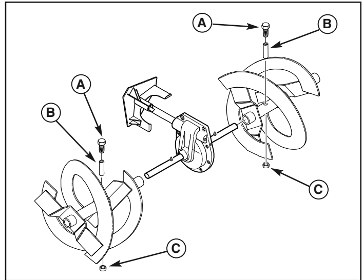
Replacing Auger Shear Bolt
