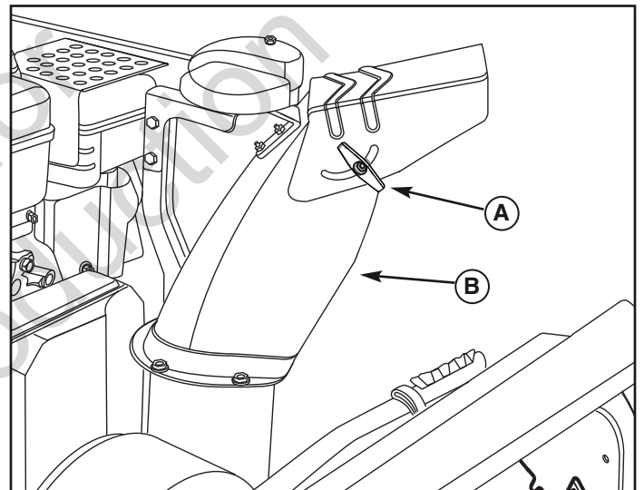
Setting the Chute Deflector Angle
