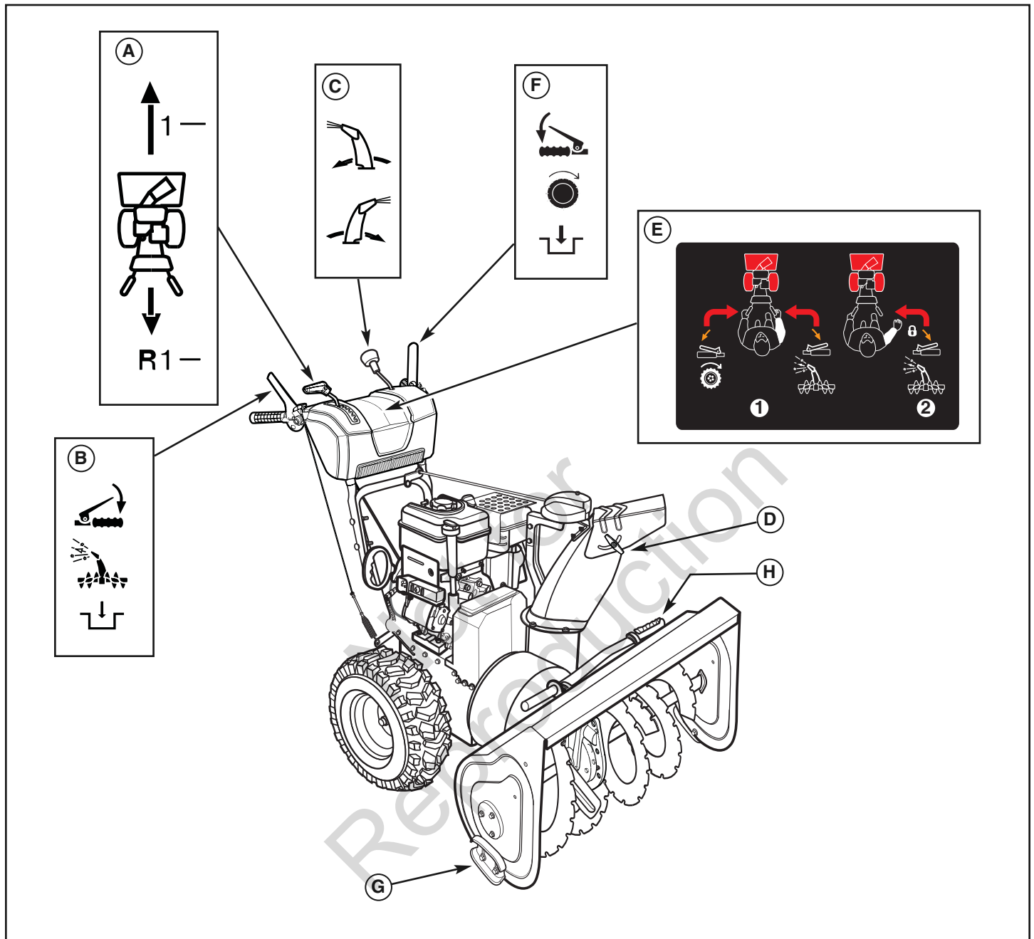
Snowthrower Controls
