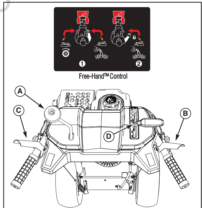
Control Levers
